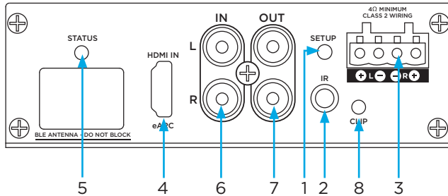
UA 2-125 ARC Amplifier Audio Connector Panel
